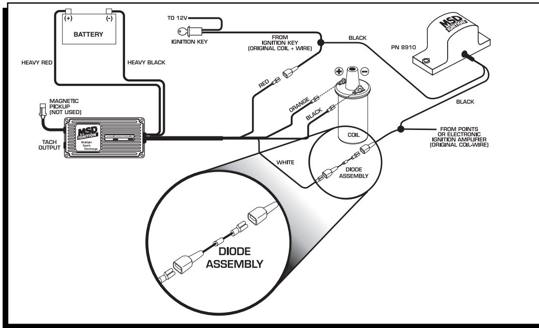
Figure 2 Wiring With the Diode Assembly.
