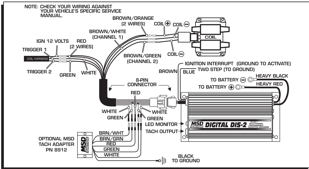
Figure 2 Typical Installation with an MSD DIS-2 Ignition.
