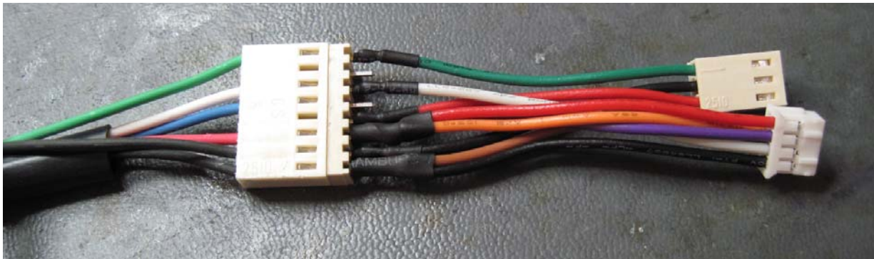
Figure 1. Adapter Harness Connected to Digital Gauge Harness
