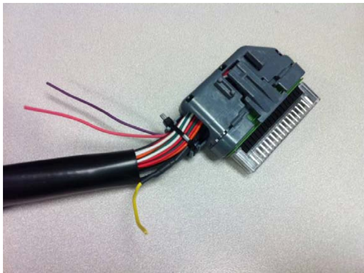
FIGURE 9. Mode Configuration Wires
