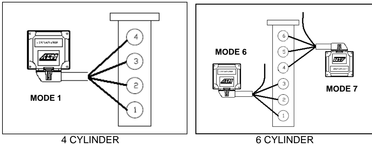
FIGURE 8. 4 CH UEGO controller configuration mode
