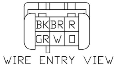
FIGURE 17. UEGO Connector Pin-out
