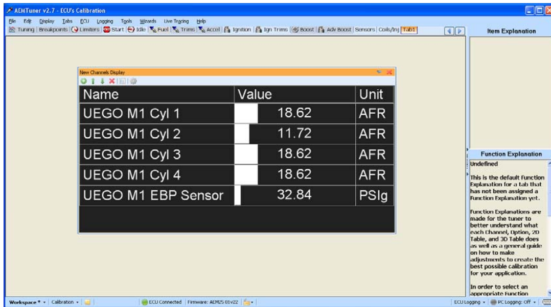
FIGURE 14. Mode 1 + EBP Sensor
